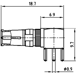
Socket contact
