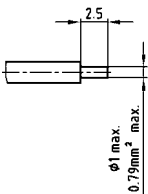
Wire stripping
