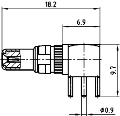
Plug contact
