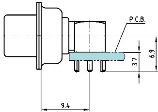
Installation dimension
