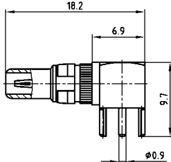
Plug contact
