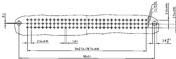
Panel cutout
