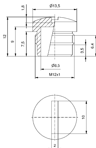
DIMENSION DRAWING
