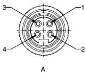
4-pos female
