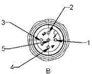
5-pos male
