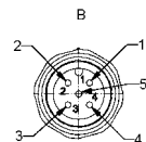
5-pos male
