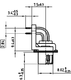
Shell size 1-4
