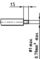
Wire stripping
