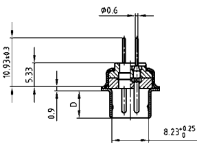
Shell size 1-4
