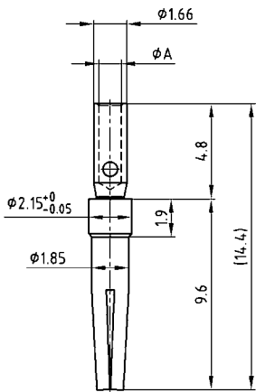
Signal socket crimp contact (Standard version)
