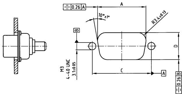
Rear panel mounting
