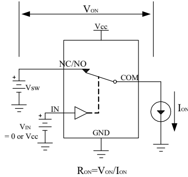
Figure 2 Switch on resistor
