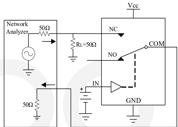
Figure 7 Off-isolation
