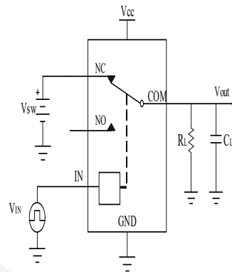
Figure 9 Turn-On/Turn-Off
