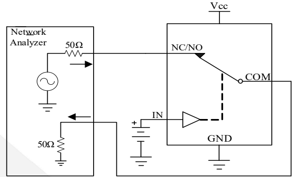
Figure 5 Bandwidth
