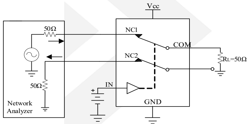
Figure 6 Channel-to-channel crosstalk
