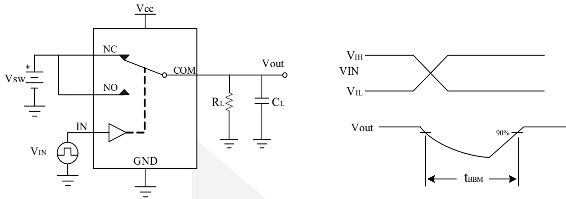
Figure 8 Break-Before-Make
