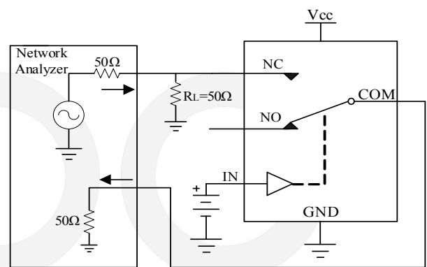
Figure 7 Off-isolation
