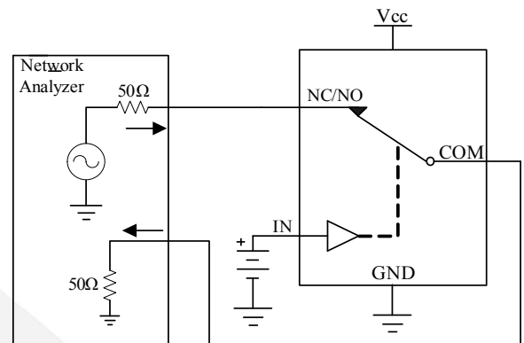
Figure 5 Bandwidth
