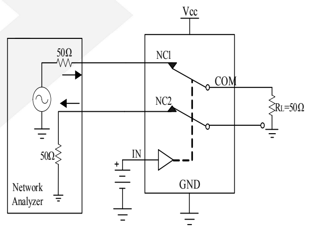
Figure 6 Channel-to-channel crosstalk
