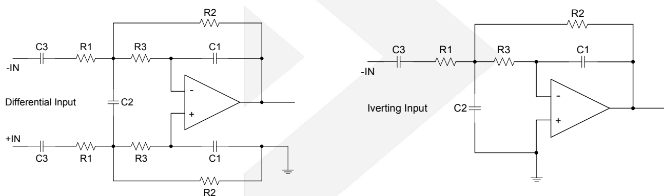
Figure 3 Second-Order Active Low-Pass Filter
