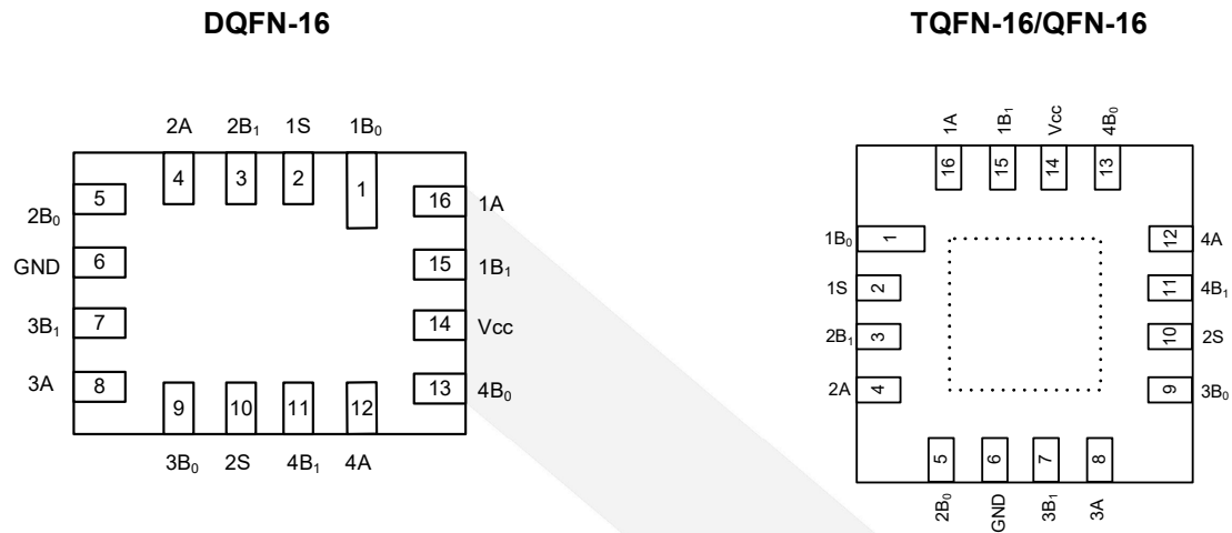
Figure 1 Top View
