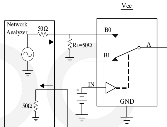
Figure 7 Off-isolation
