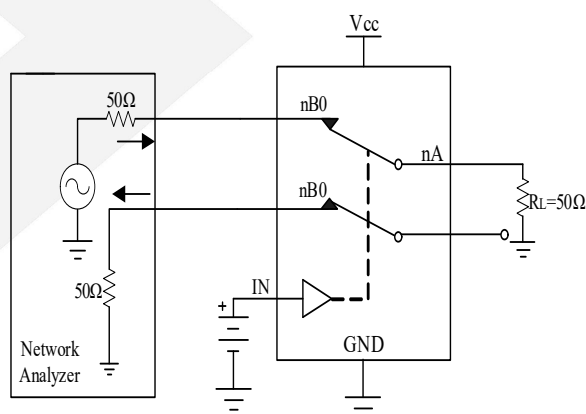
Figure 6 Channel-to-channel crosstalk
