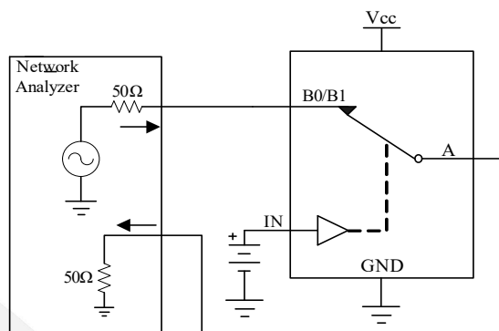
Figure 5 Bandwidth
