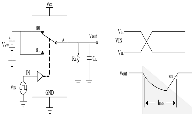
Figure 8 Break-Before-Make
