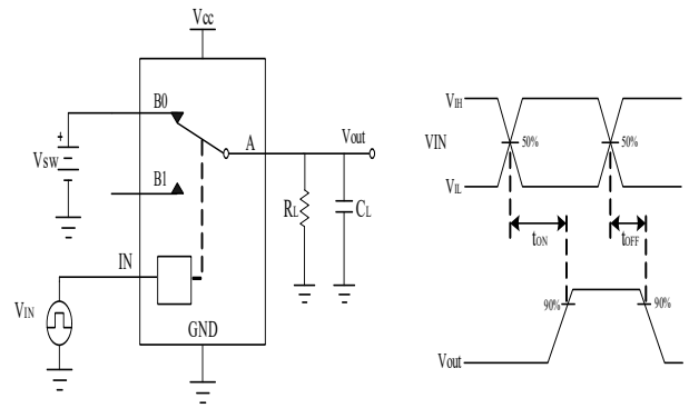
Figure 9 Turn-On/Turn-Off
