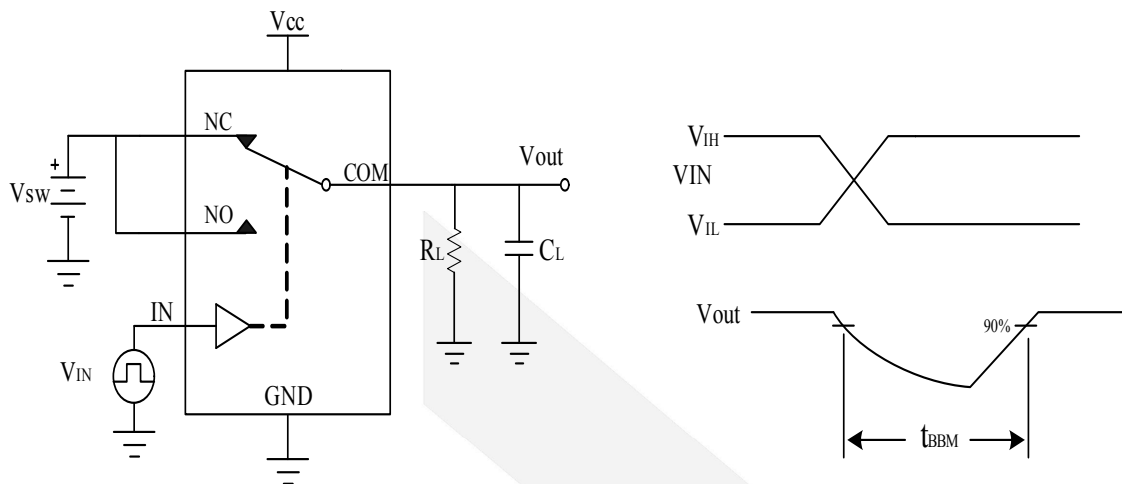
Figure 8 Break-Before-Make
