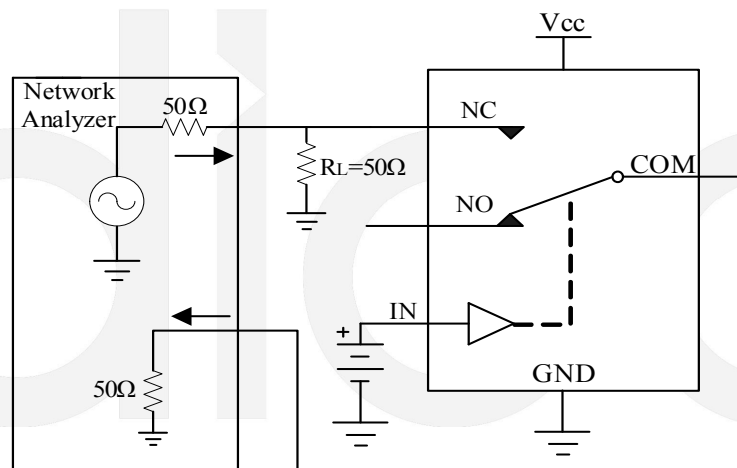
Figure 7 Off-isolation
