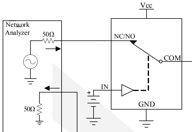
Figure 5 Bandwidth
