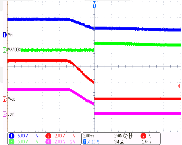
VIN Power OFF ( V_{IN}=5V , R_{Load}=1.6\Omega )
