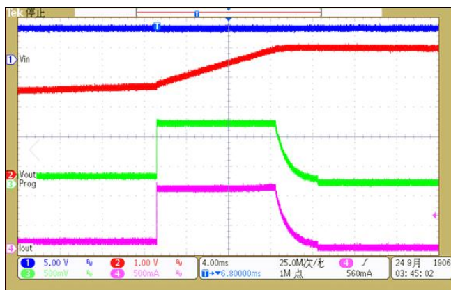
Charging curve
