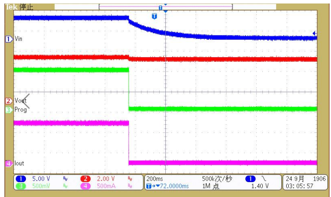
V CC Shut-down
