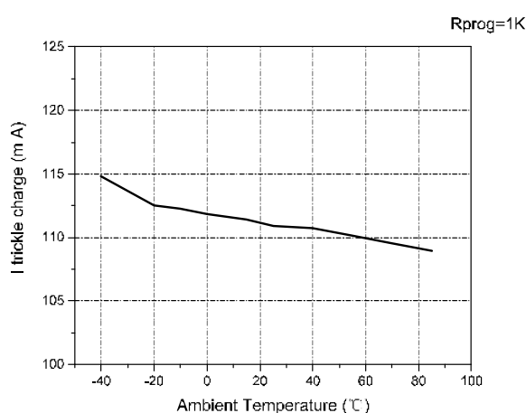
Trickle charge current vs. Ambient temperature
