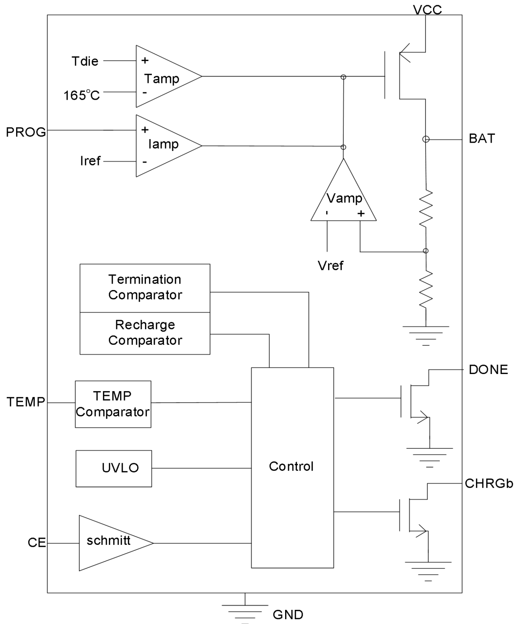
Figure 3. Block diagram
