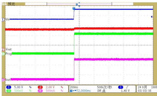
V CC Start-up
