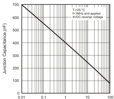
Fig.5- Junction Capacitance
