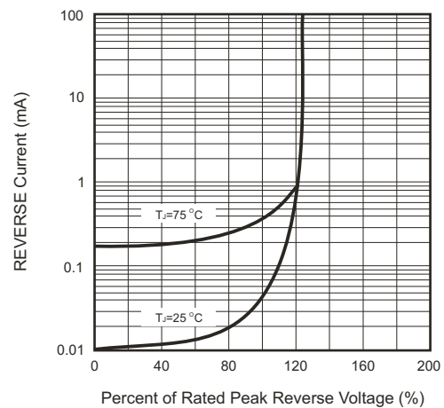
Fig.4- Reverse Characteristics
