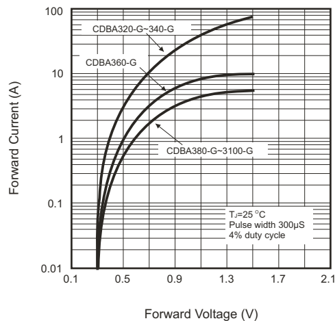
Fig.3- Forward Characteristics
