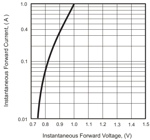
Fig.1-Typical Forward Characteristics
