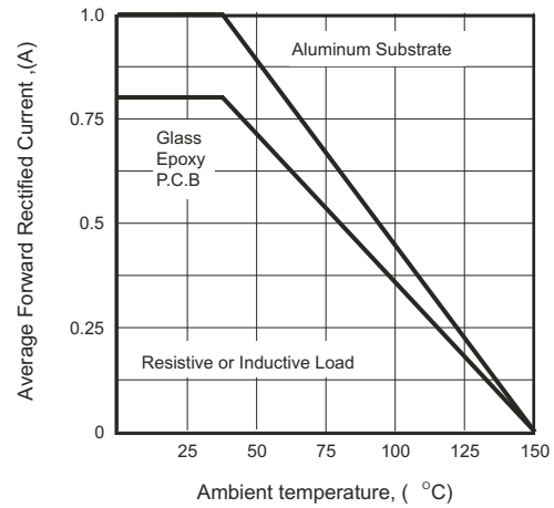
Fig.2-Forward Derating Curve
