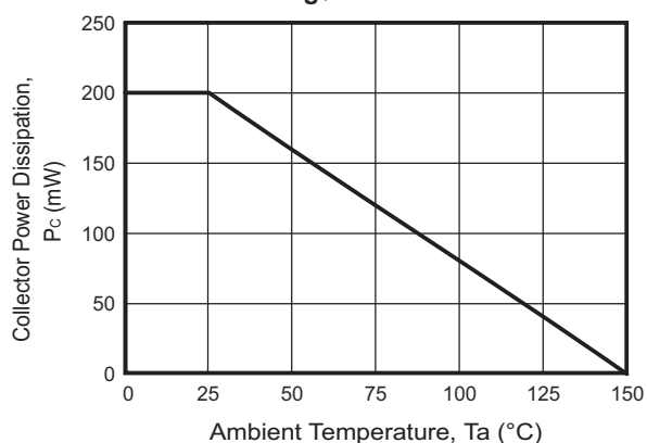
Fig.8- P_c — T_a
