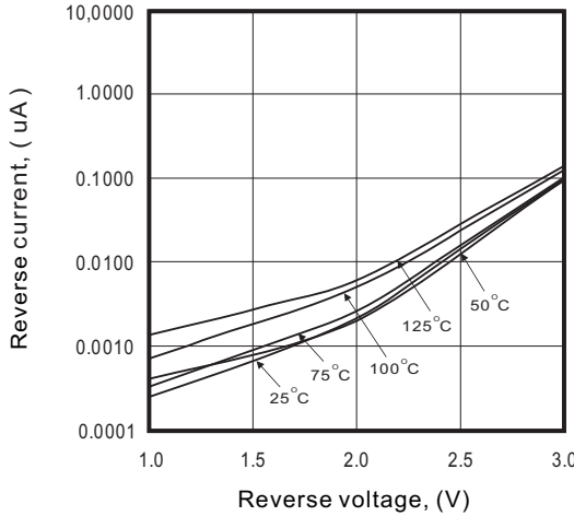
Fig.2 - Reverse characteristic
