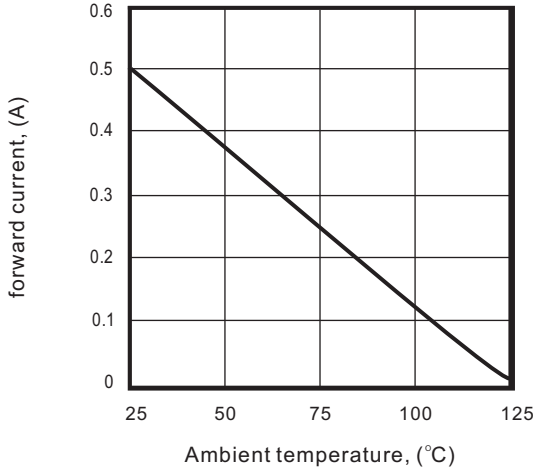
Fig.4 - Power derating
