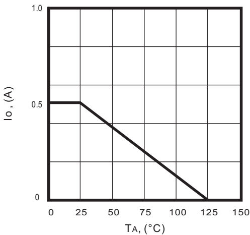
Fig.4 - Derating curve
