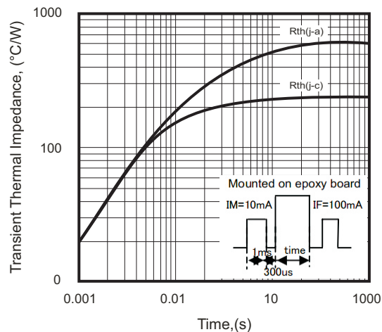
Fig.5 - Rth-t Characteristics
