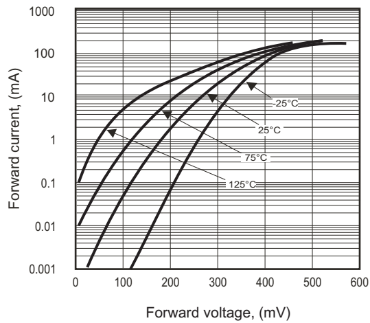
Fig.1 - Forward Characteristics
