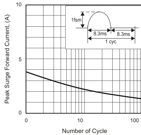
Fig.4 - IFSM-Cycle Characteristics
