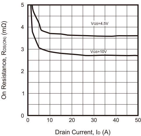
Fig.2 - On-Resistance vs. Drain Current
