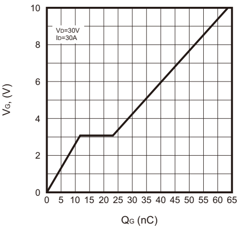
Fig.6 - Gate-Charge Characteristics
