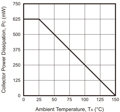
Fig.8 - P_c — T_A
