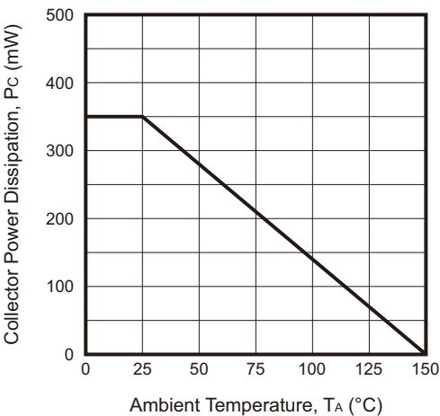
Fig.8 - P_C — T_A
