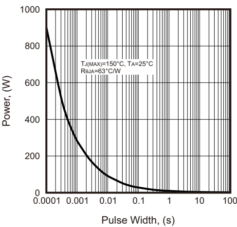
Fig.13 - Single Pulse Power Rating, Junction to Ambient
