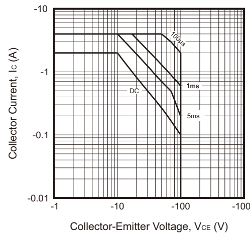
Fig.6 - Safe Operating Area
