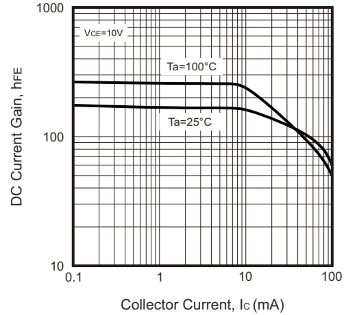
Fig.2 - h_{FE} — I_C
