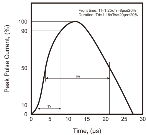
Fig.2 - Pulse Waveform
