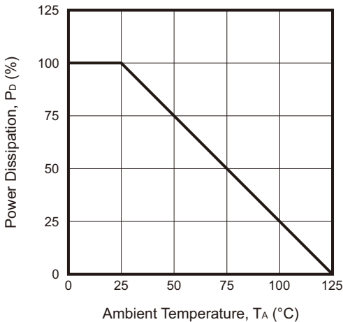
Fig.4 - Derating Curve ( P_D - T_A )
