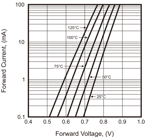
Fig.5 - Forward Characteristic
