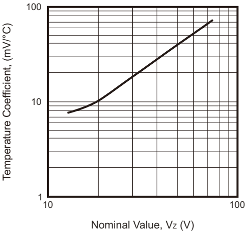
Fig.2 - Temperature Coefficient
