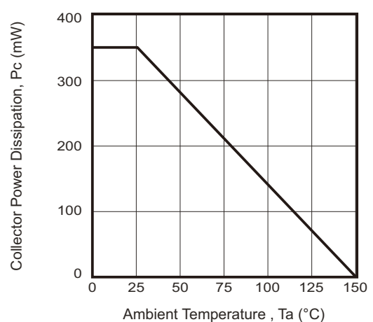
Fig.8 - P_C — T_a
