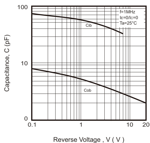
Fig. 7 - C_{ob}/C_{ib} — V_{CB}/V_{EB}
