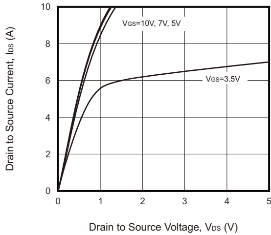
Fig.1 - Output Characteristic
