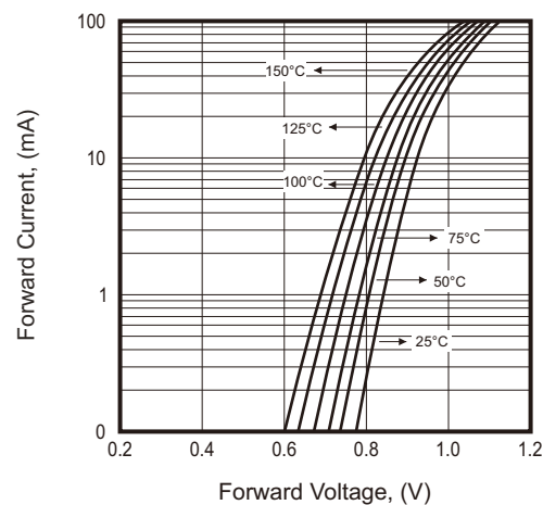
Fig.4 - Forward Characteristic
