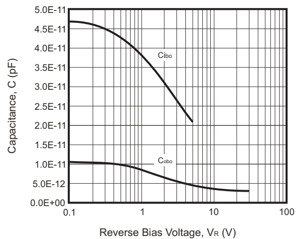
Fig.6 - Capacitance
