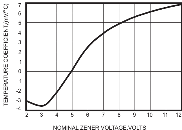
Fig.1 TEMPERATURE COEFFICIENTS
