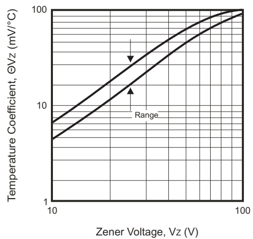
Fig.2 - Temperature Coefficients v.s. Zener Voltage
