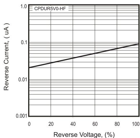
Fig.2-3 - Reverse Characteristics
