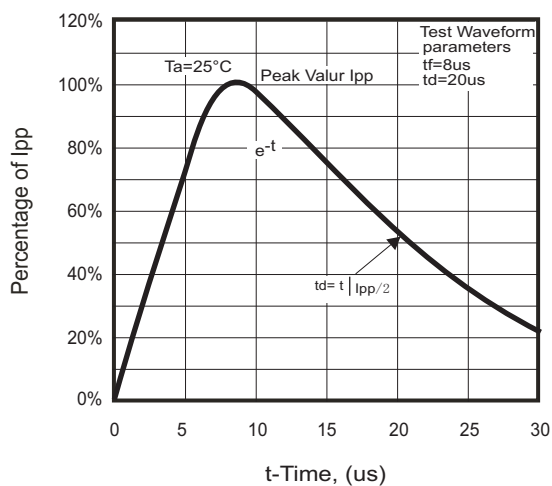
Fig.1 - Pulse Waveform
