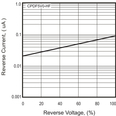
Fig.2-3 - Reverse Characteristics
