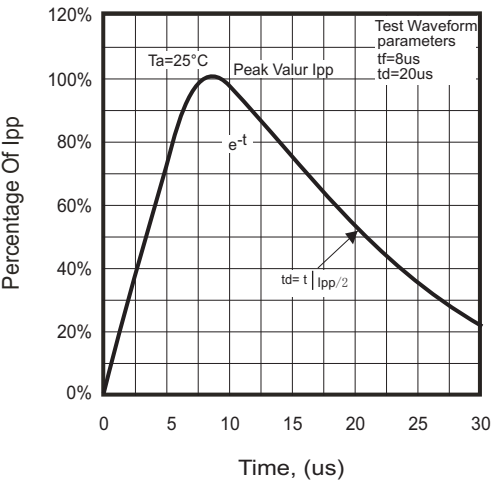
Fig.1 - Peak Pulse Current Wave Form Acc. IEC 61000-4-5
