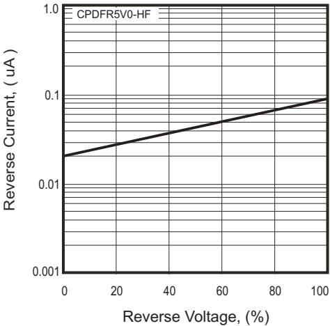
Fig.2-3 - Reverse Characteristics
