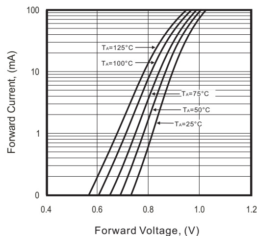
Fig.2 - Forward Characteristics
