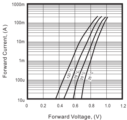
Fig.1 - Forward Characteristics
