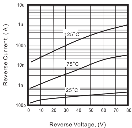
Fig.2 - Reverse Characteristics
