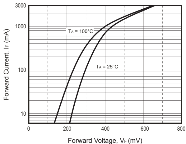
Fig.3 - Forward Characteristics
