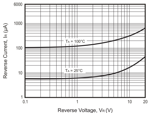
Fig.4 - Reverse Characteristics
