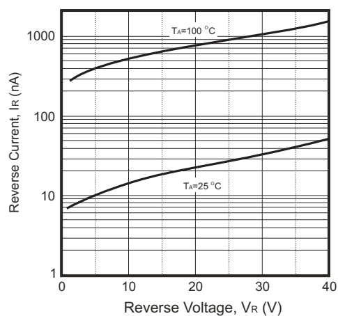
Fig.2 - Reverse Characteristics
