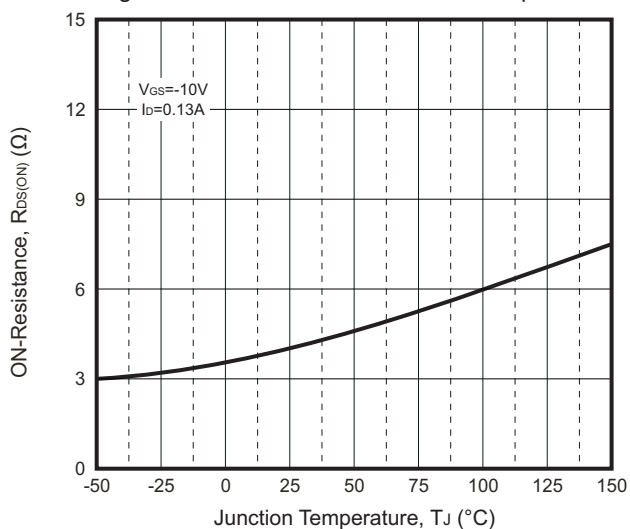
Fig.5 - ON-Resistance vs. Junction Temperature
