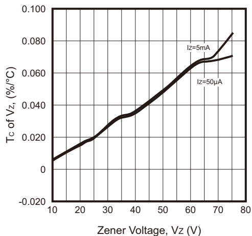
Fig.7 - Typical Temperature Coefficient of Zener Voltage
