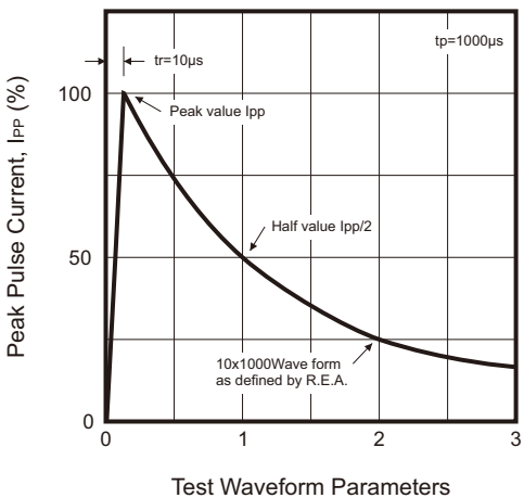
Fig.2 - Pulse Waveform
