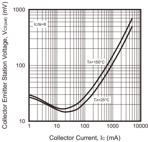
Fig.2 - V_{CE(sat)} vs. I_c
