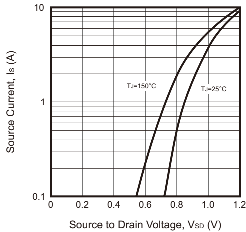
Fig.7 - Source Drain Diode Forward Voltage
