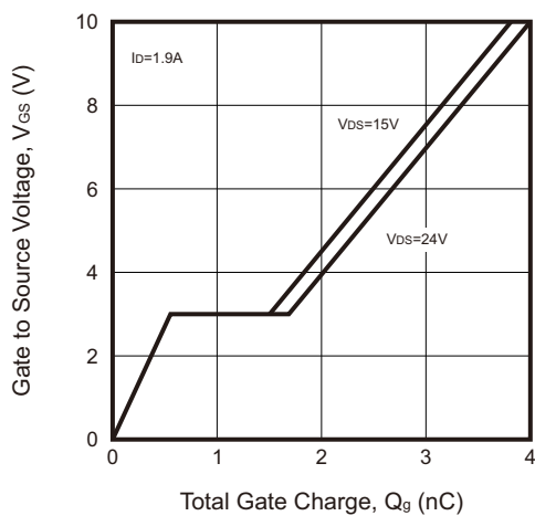
Fig.5 - Gate Charge
