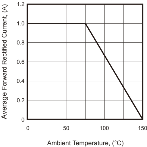
Fig.1 - Max. Average Forward Current Derating
