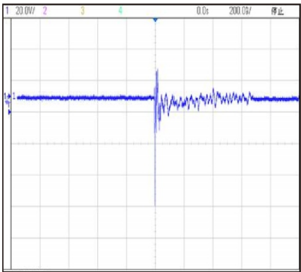
Fig.7 - -8kV Contact IEC 61000-4-2
